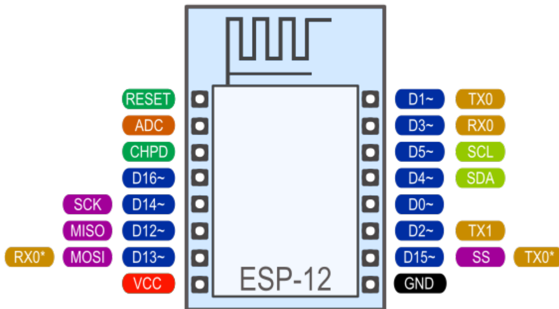
Fig. 1: Pin Functions
